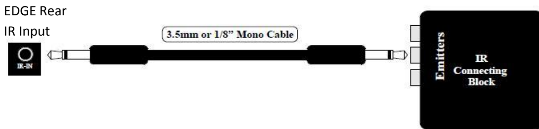
Figure 2: Illustration of IR connecting block to EDGE IR input
