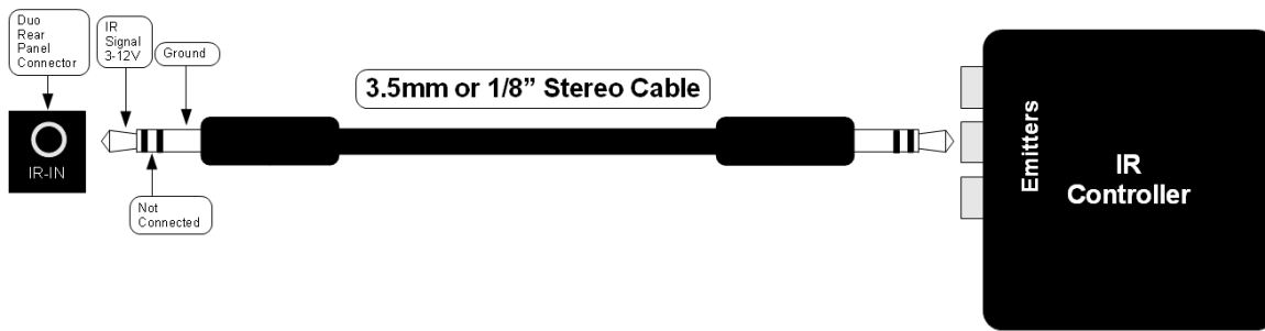
Figure 5: IR controller connection to the iScan Duo IR input
