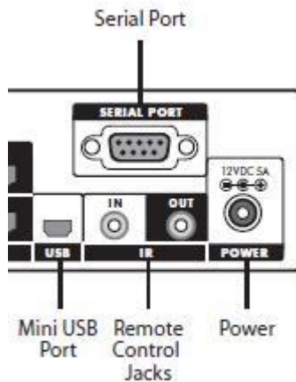
Figure 3: iScan Duo rear panel IR Jacks
